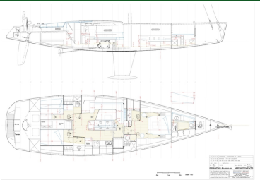
NEREIDE Custom Sailing Yacht 64 (2005)
