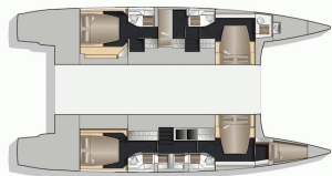
NAUTITECH 542 DESIGN BY WINDWARD ISLANDS CONSTRUCTION BY NAUTITECH SHIPYARD
