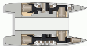
NAUTITECH 542 DESIGN BY NAUTITECH SHIPYARD CONSTRUCTION BY NAUTITECH SHIPYARD
